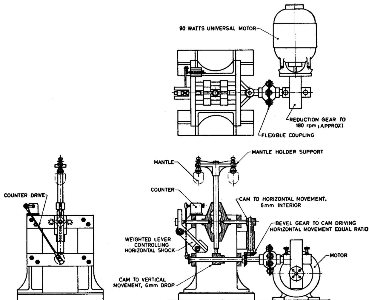
Figure 1 — Shock testing machine
