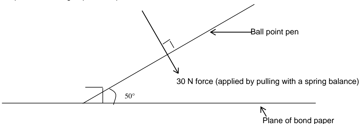
Figure 1 — Illustration for load test
