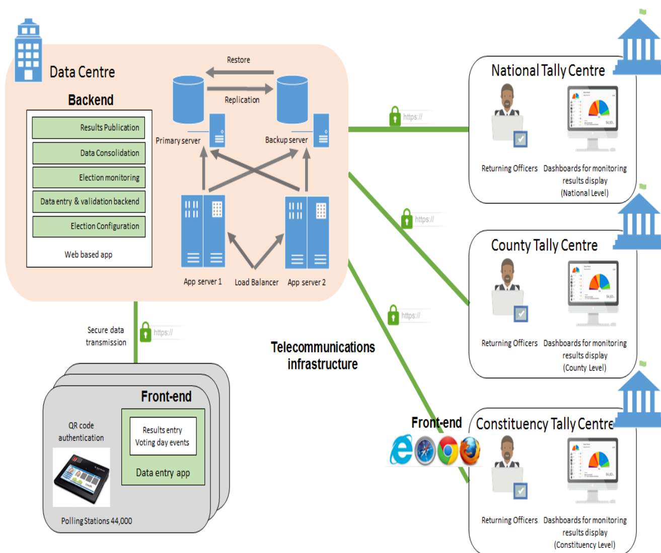
Figure 1 – Current KIEMS Network Architecture Layout
