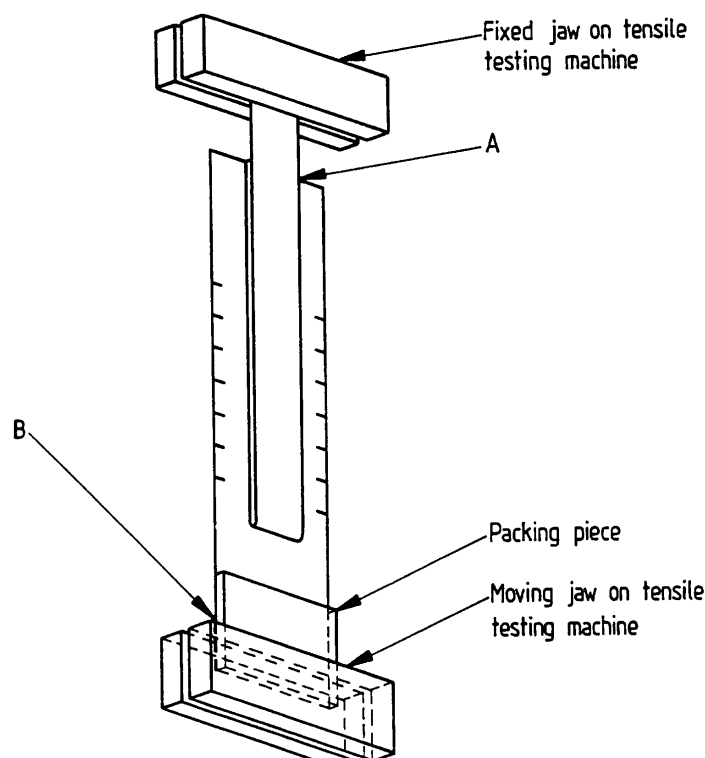
Figure 2 — Typical arrangement for stripping the tape from the plate
