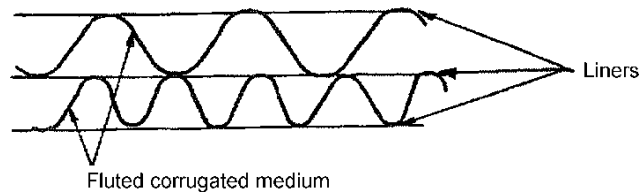
Fig. 2 — Double-wall corrugated fibreboard
