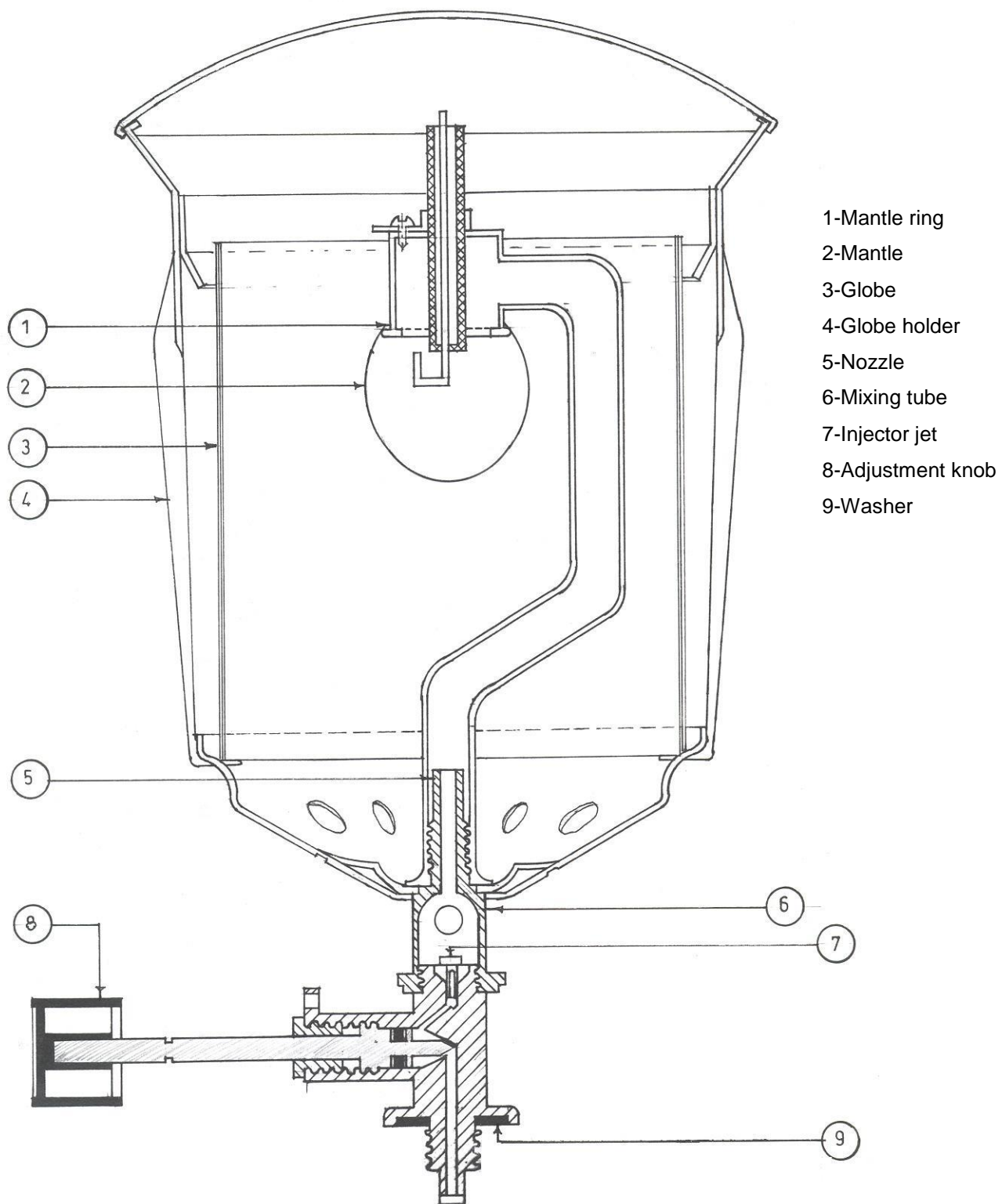
Figure 1 — Typical section through gas lamp.
